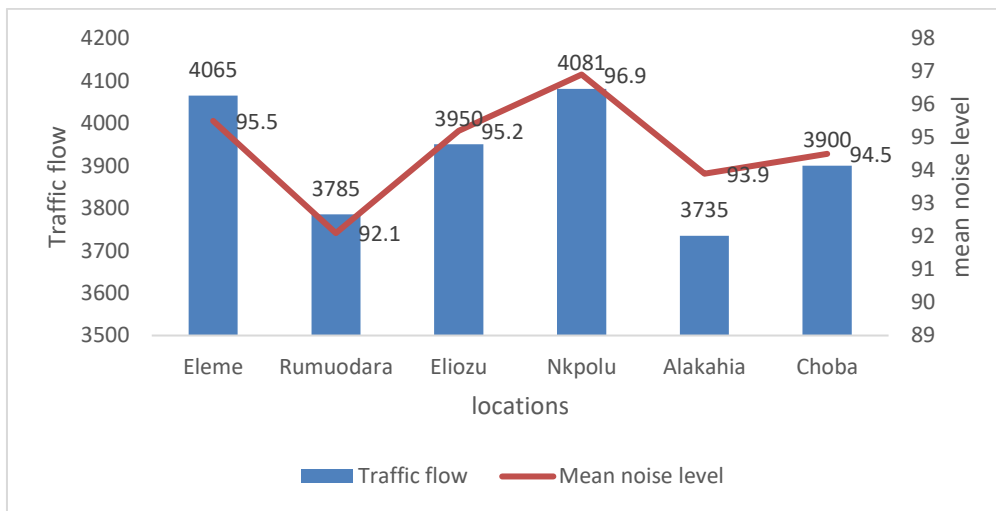
Fig. 7. Mean representation of traffic flow and noise level for peak traffic period
